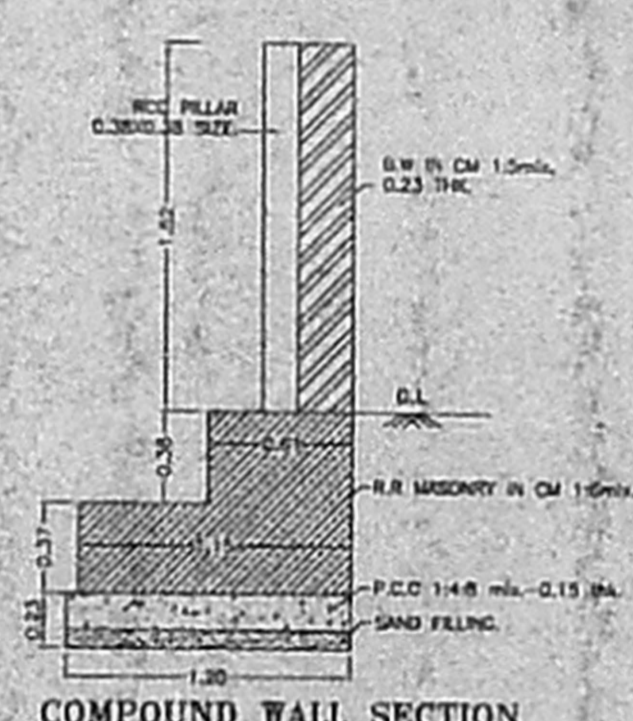
COMPOUND WALL SECTION
