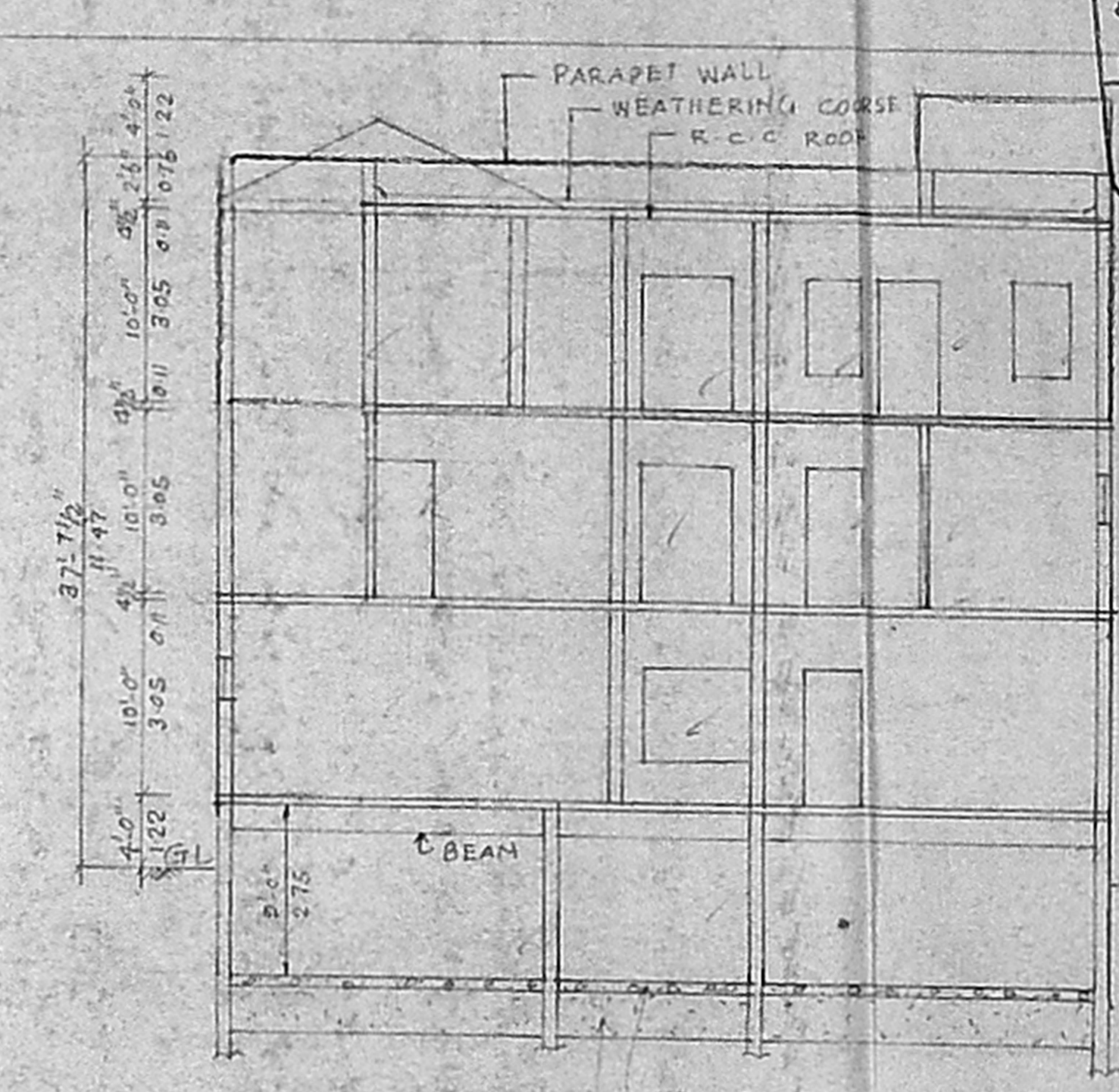
SECTION-BB BLOCK-1
